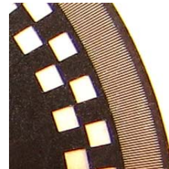
Optical Encoder Disk
